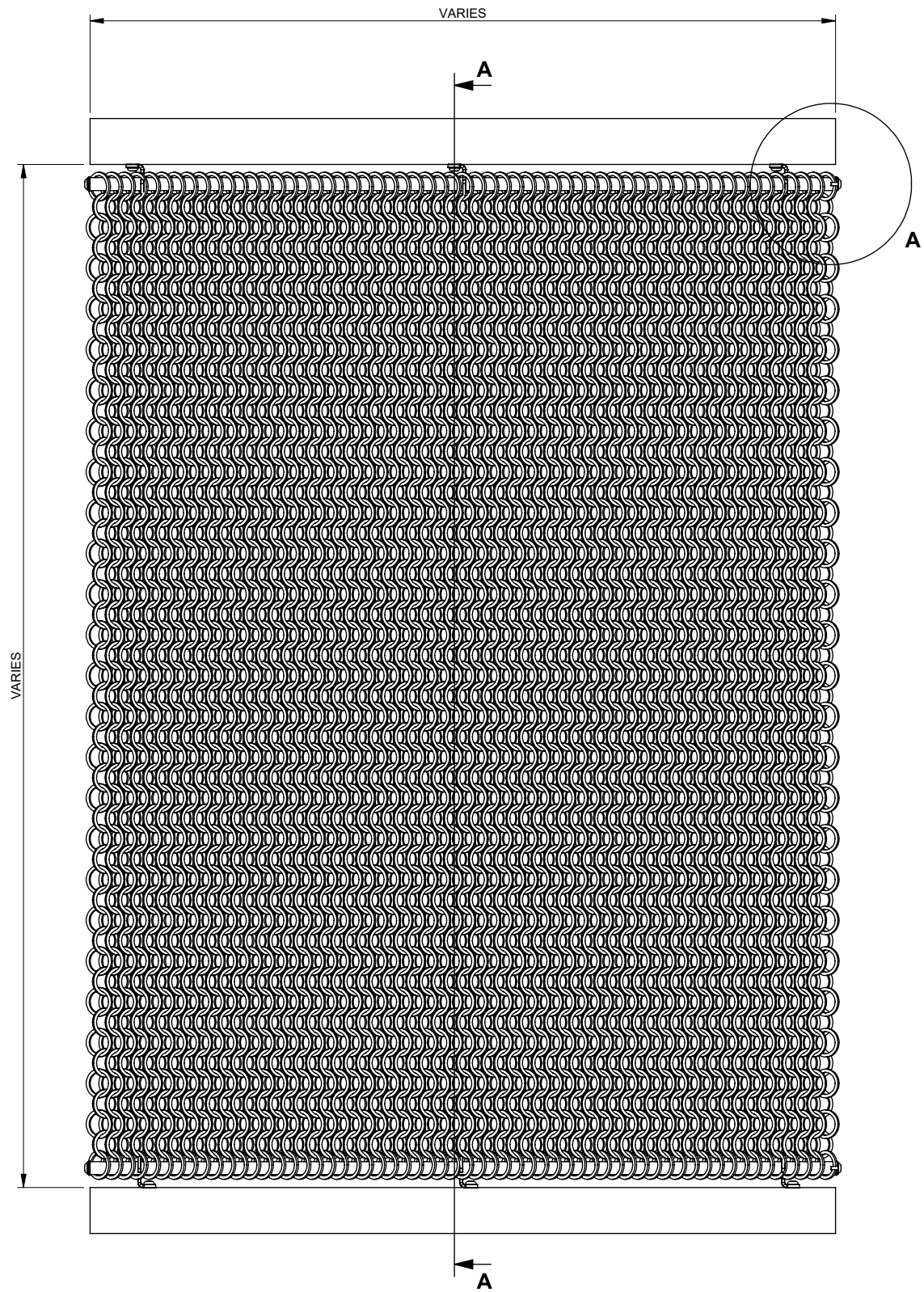
FRONT ELEVATION (TYPICAL HANGING SCREEN WITH BOTTOM FIXING)
